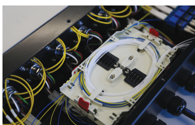
Splice cassette
