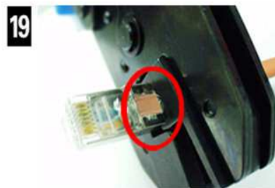
19. use crimper, clamping
