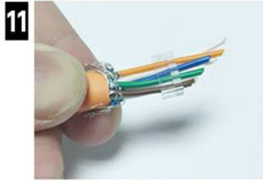
11. Wear into the line
