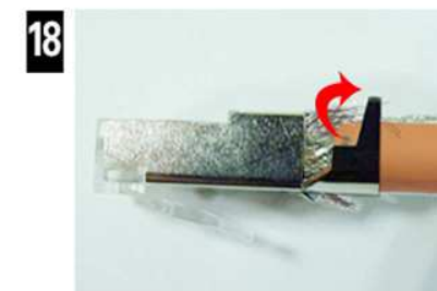
18. clamp ground wire
