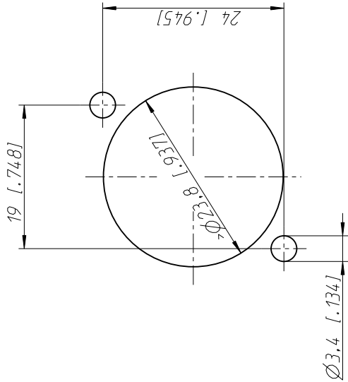
Frontplattenausschnitt (Montage von hinten) Panel cut out (Panel-mounting option rear side)
