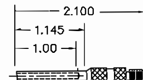
3696 - #12 PIN REMOVAL
