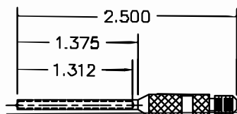
3697 - #16 PIN REMOVAL
