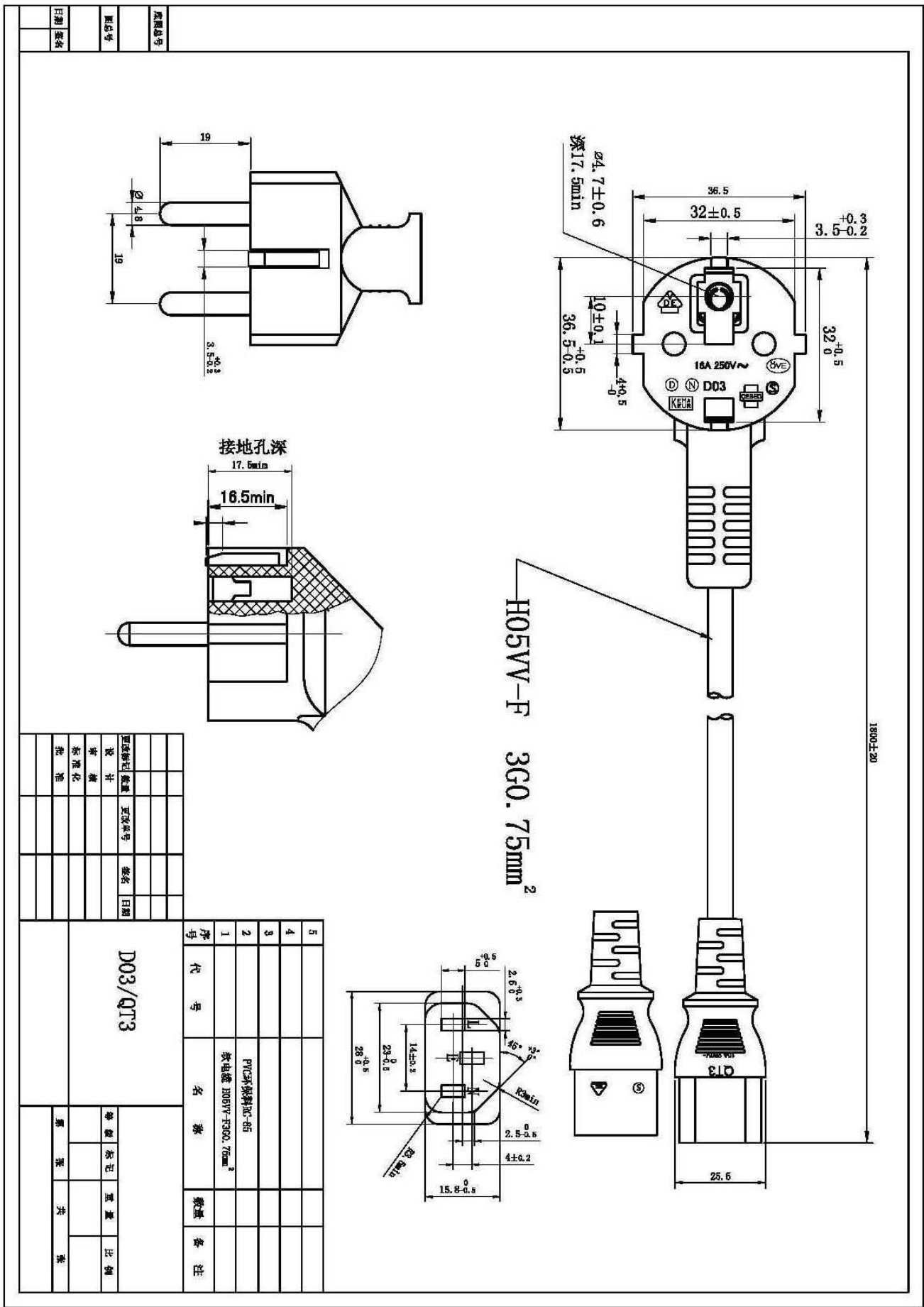
(1) Power Cord Specification (Tabel 1) Drawing 1
