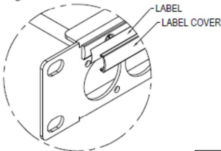
VIEW SHOWING LABEL & LABEL COVER REMOVED
