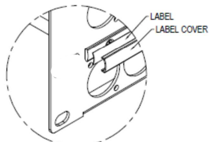
VIEW SHOWING LABEL & LABEL COVER REMOVED
