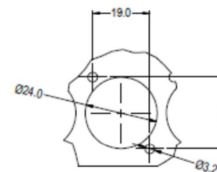
DETAIL VIEW A (32x POSITIONS)
