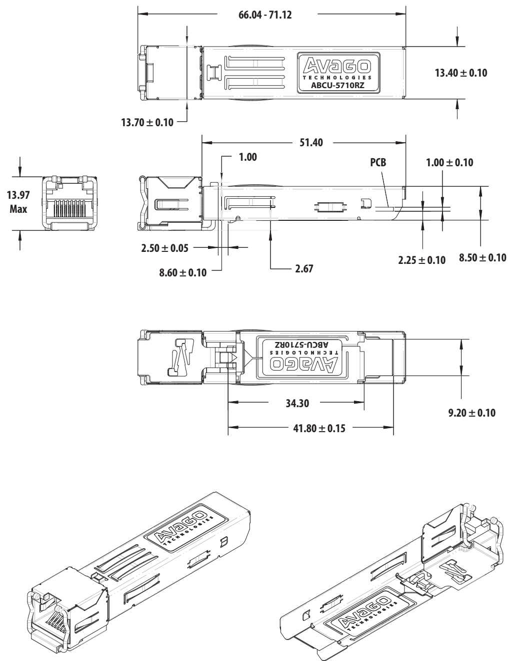
Figure 7a. Module Drawing
