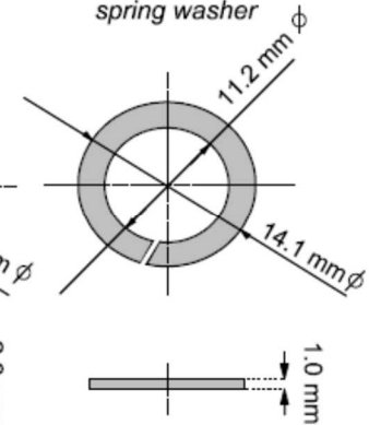
Federring spring washer
