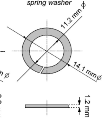
Federring spring washer
